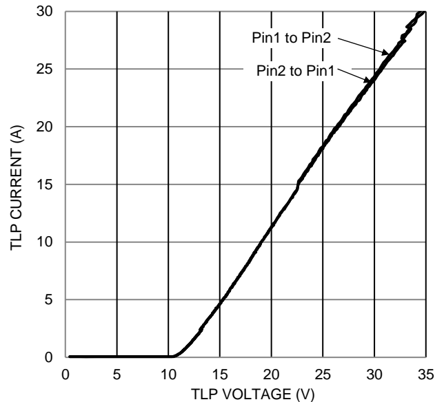
Figure 8 Transmission Line Pulsing (TLP) Current vs. Voltage
