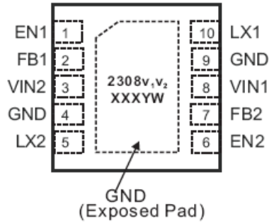
TOP VIEW WDFN-10L 3x3
