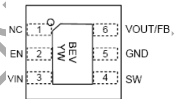
Top View DFN 2x2 6L
