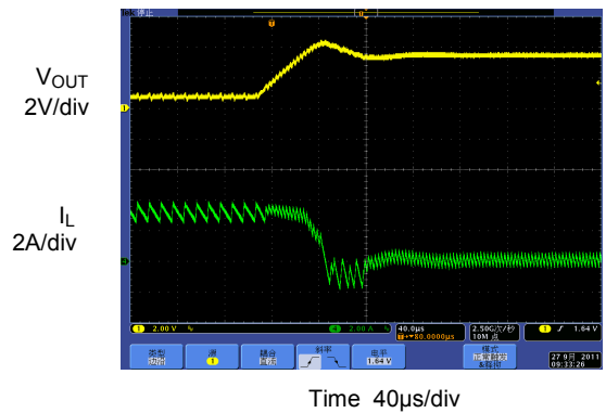
Short Circuit Recovery ( I_{OUT}=0\text{A} )
