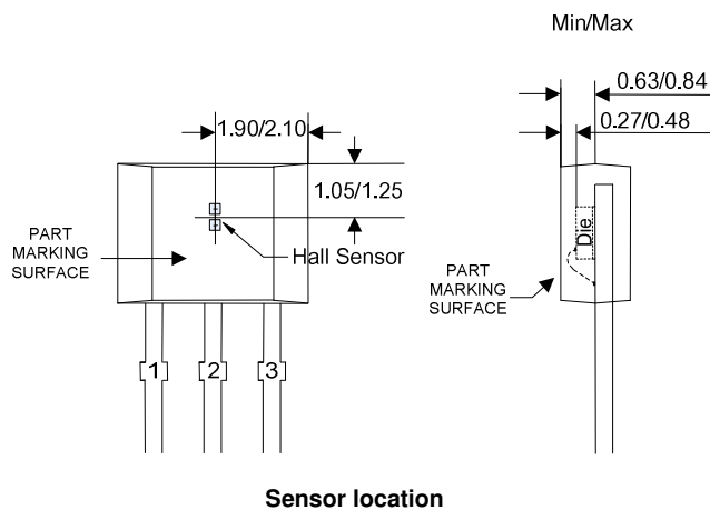
Sensor location
