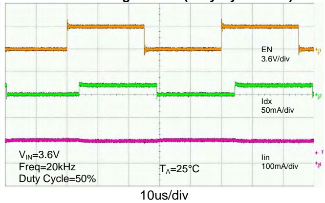
PWM Dimming Control (Duty Cycle=50%)
