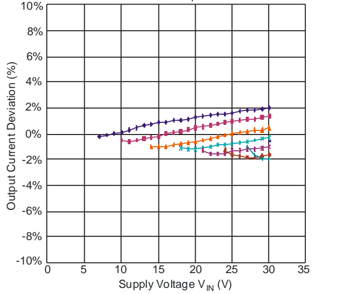
ZXLD1360 Output Current L = 100μH
