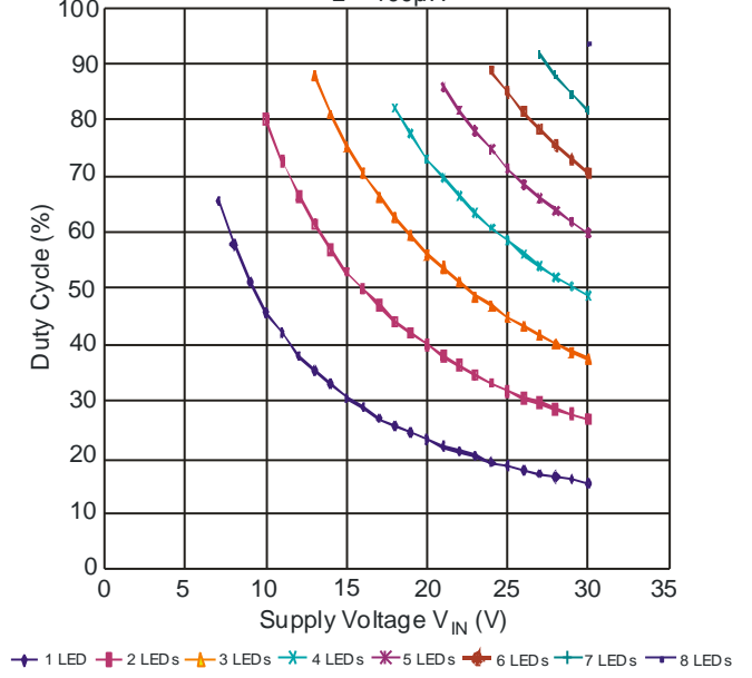
ZXLD1360 Duty Cycle L = 100μH
