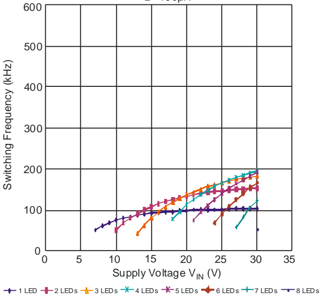
ZXLD1360 Switching Frequency L = 100μH
