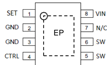
MSOP-8EP
