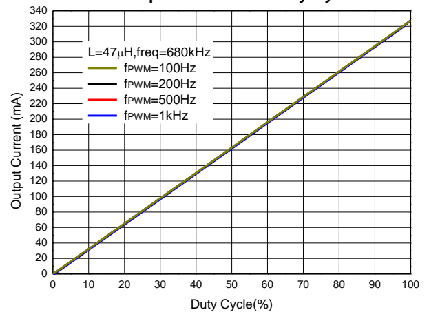
PWM Dimming (V IN =16V, 3LEDs, 47μH, R S =0.3Ω) Output Current vs. Duty Cycle
