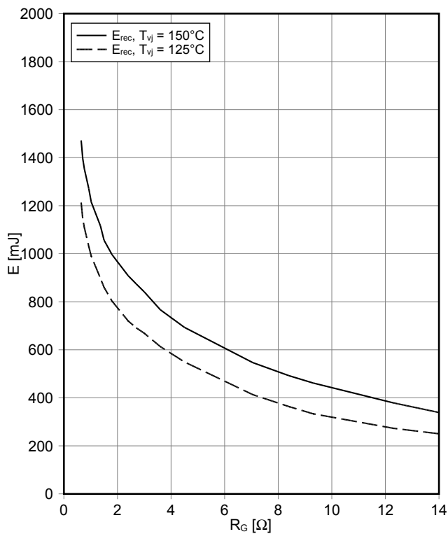
Schaltverluste Diode, Revers (typisch) switching losses Diode, Reverse (typical) E_{rec} = f(R_G) I_F = 1000 \text{ A}, V_{CE} = 1800 \text{ V}
