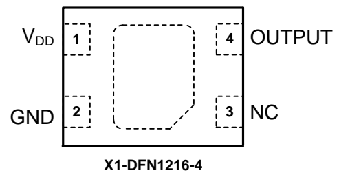
X1-DFN1216-4
