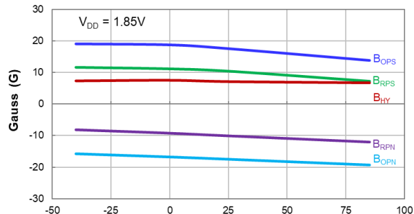
Switch Points B OPS and B RPS vs Temperature
