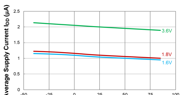
Average Supply Current vs. Temperature
