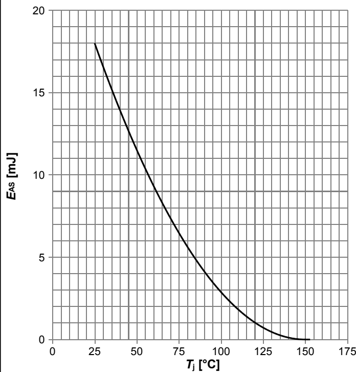
Diagram 11: Avalanche energy
