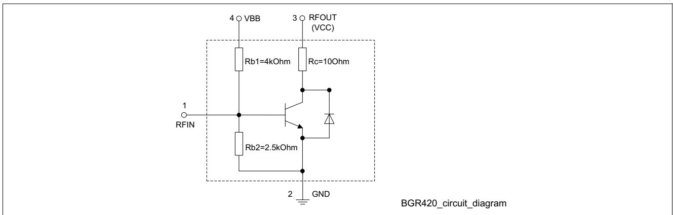
Figure 1 Circuit diagram
