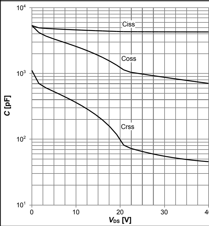
Diagram 11: Typ. capacitances
