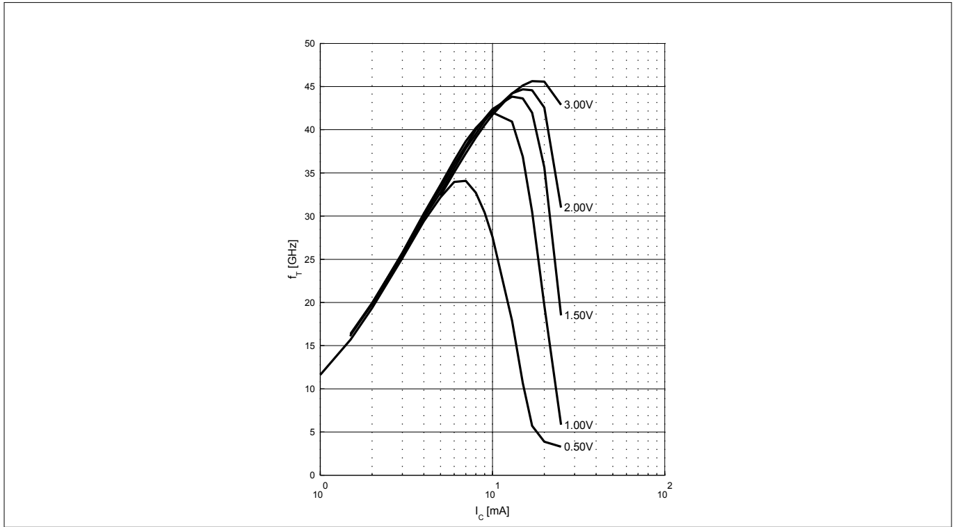
Figure 5 Transition frequency f_T = f(I_C, V_{CE}) , f = 1 \text{ GHz} , V_{CE} = \text{parameter}
