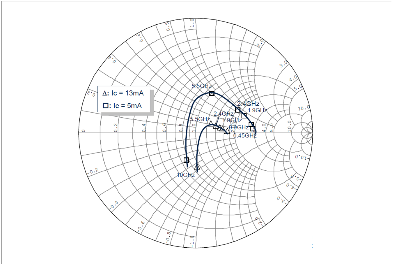
Figure 11 Source impedance for minimum noise figure Z_{s,opt} = f(f) , V_{CE} = 3\text{V} , I_C = 5 / 13\text{mA}
