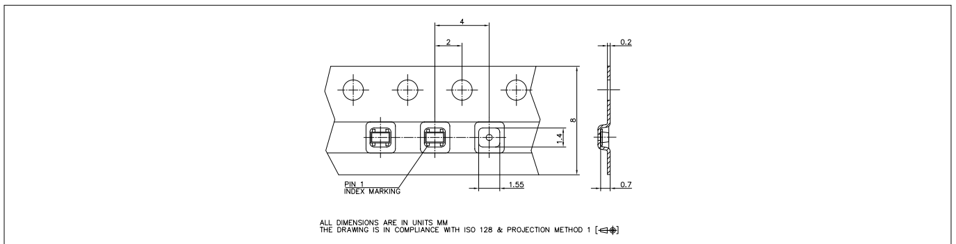
Figure 17 Tape dimensions
