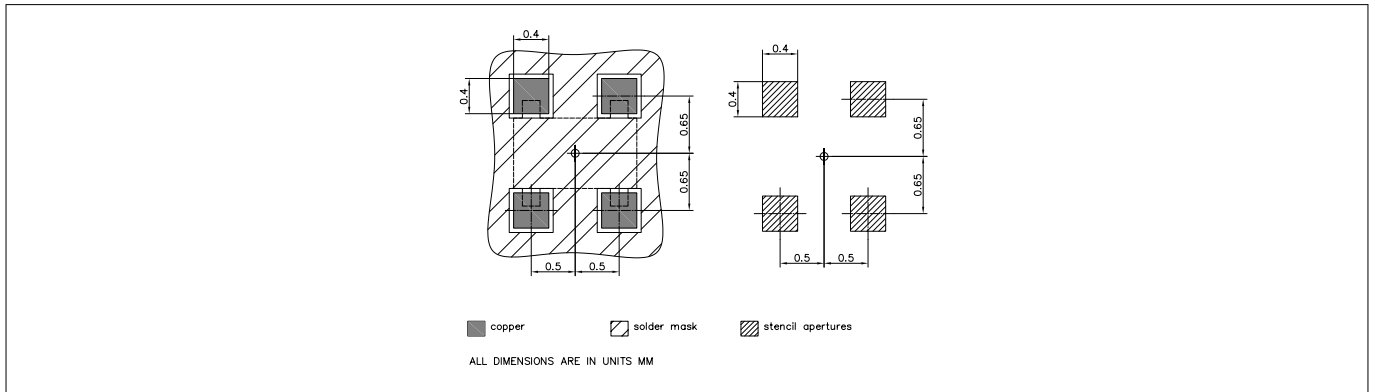
Figure 15 Foot print
