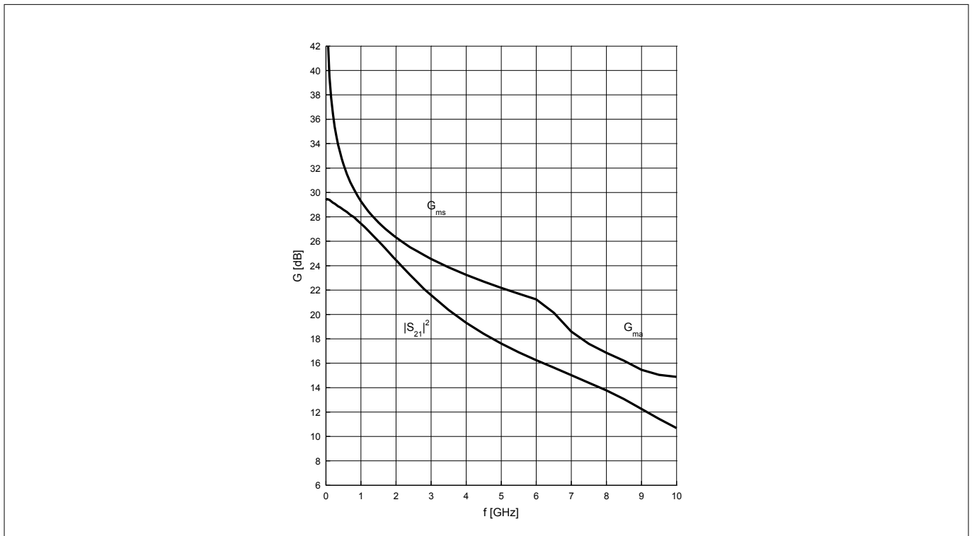
Figure 6 Power gain G_{ma} , G_{ms} , |S_{21}|^2 = f(f) , V_{CE} = 3 \text{ V} , I_C = 13 \text{ mA}
