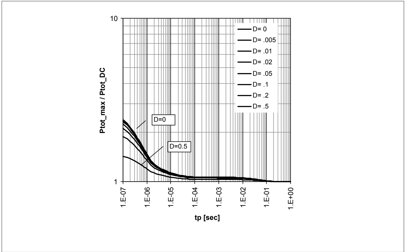
Figure 2 Permissible pulse load P_{tot\_max} / P_{tot\_DC} = f(t_p)
