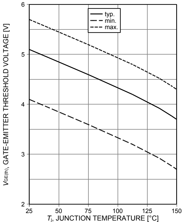
Figure 11. Gate-emitter threshold voltage as a function of junction temperature ( I_{\text{C}}=0.58\text{mA} )
