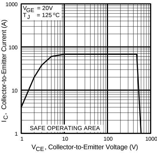
Fig. 12 - Turn-Off SOA
