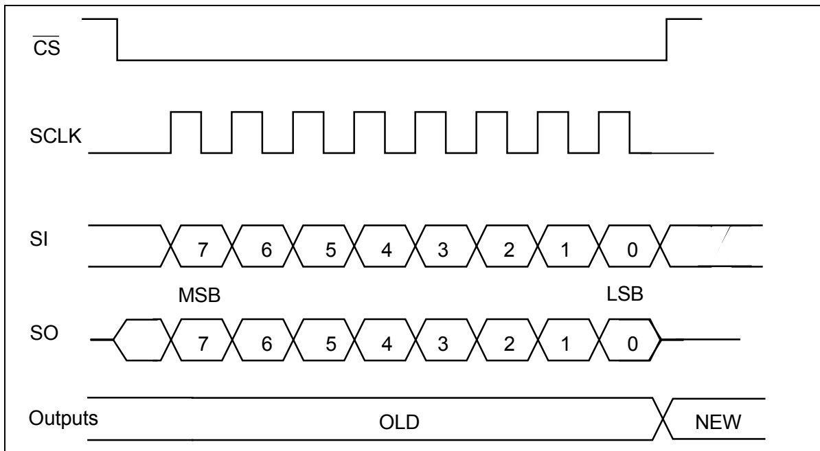
Figure 2: Serial Interface
