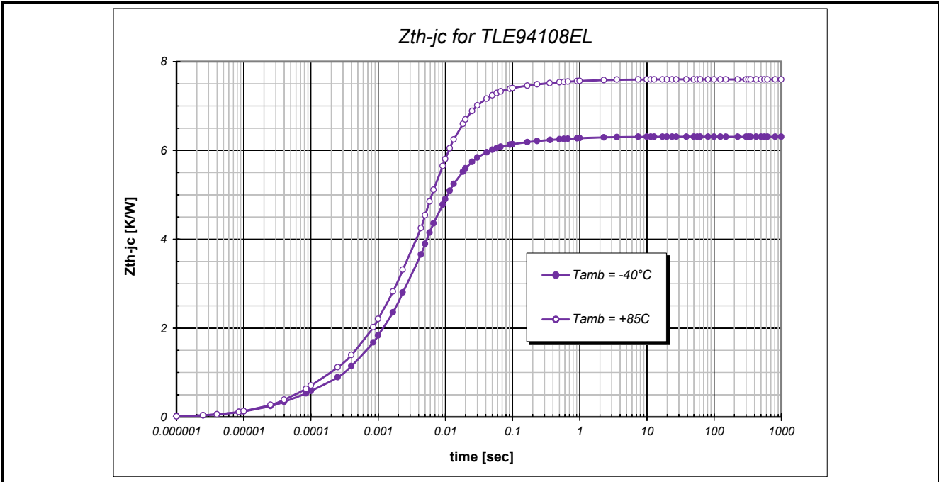
Figure 30 ZthJC Curve
