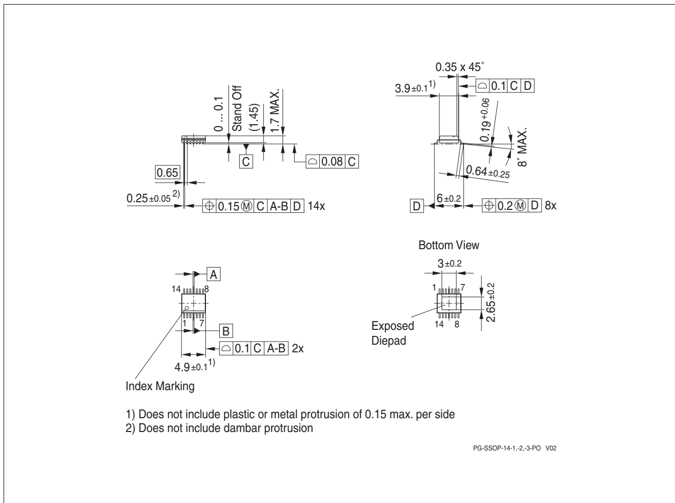
Figure 16 Package Outline PG-SSOP-14
