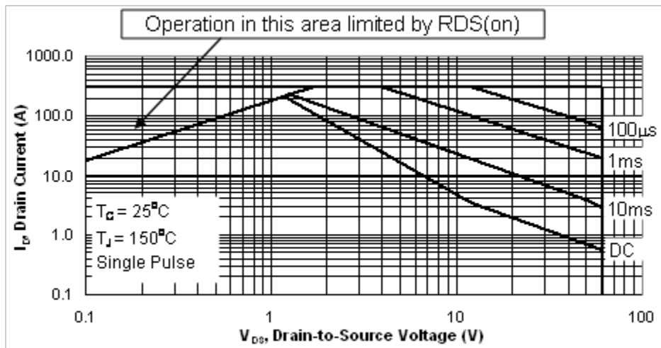
* FIGURE 4. Safe operating area graph.
