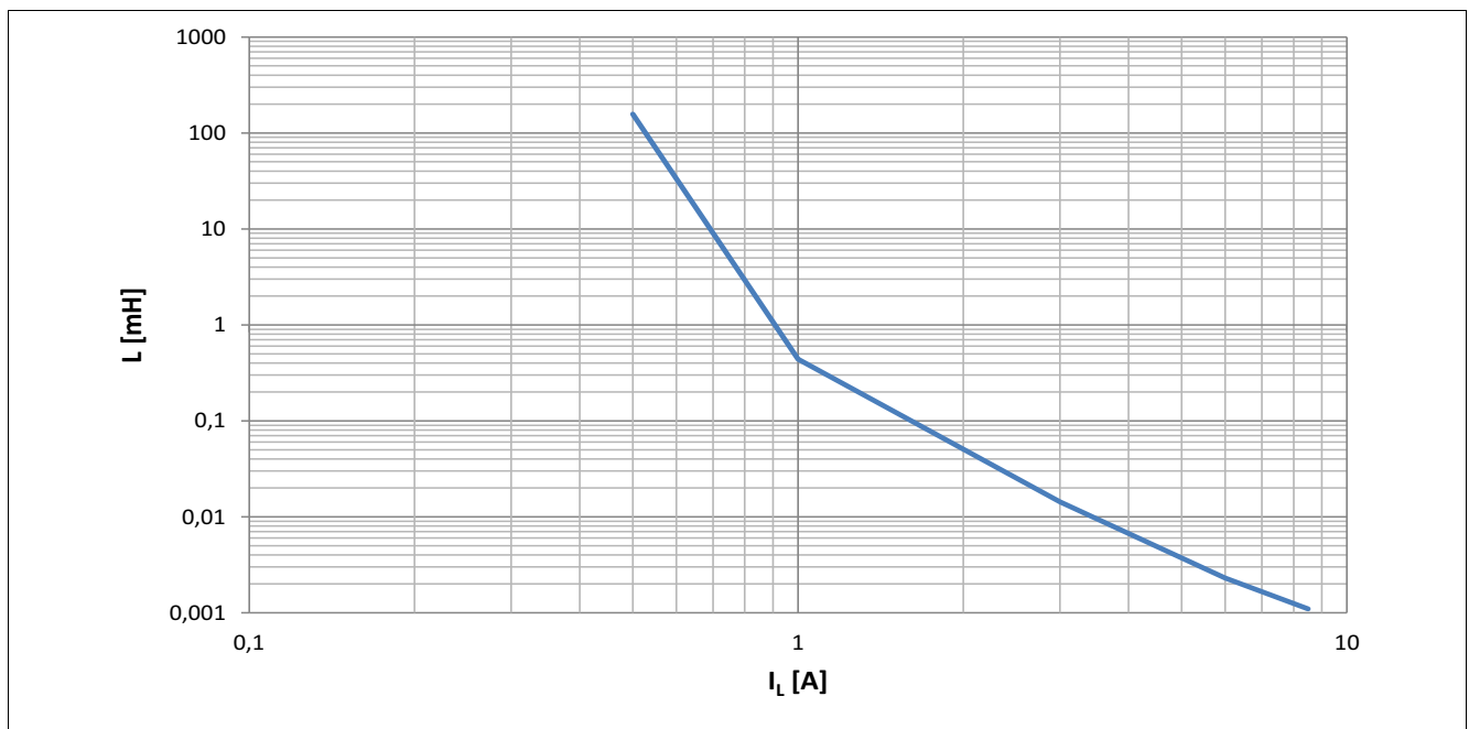
Figure 13 Maximum load inductance for single pulse L = f(I_L) , T_{j(0)} = T_{J, start} = 150^\circ\text{C} , V_{BAT} = 13.5\text{ V}
