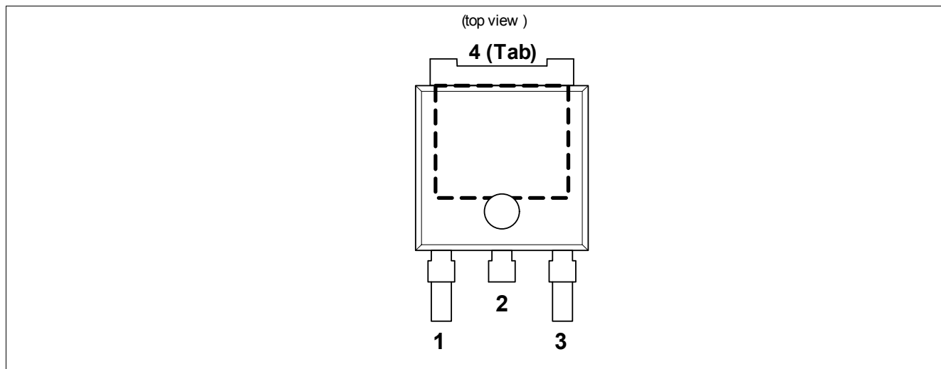
Figure 2 Pin Configuration TO252-3
