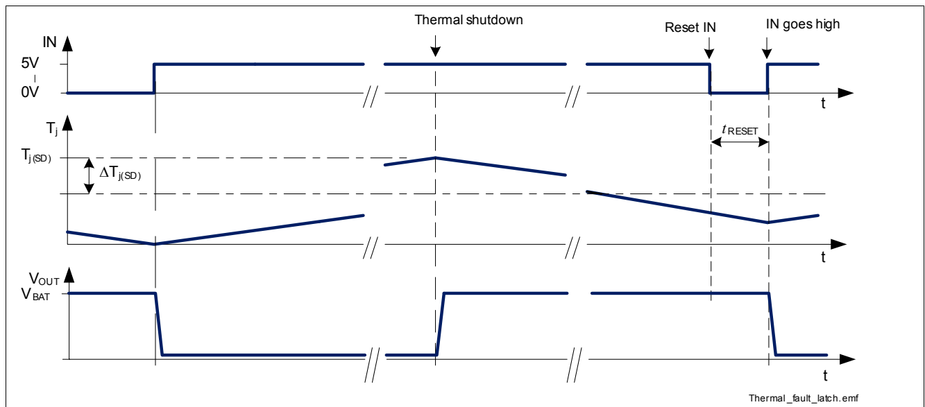
Figure 14 Thermal protective switch OFF scenario
