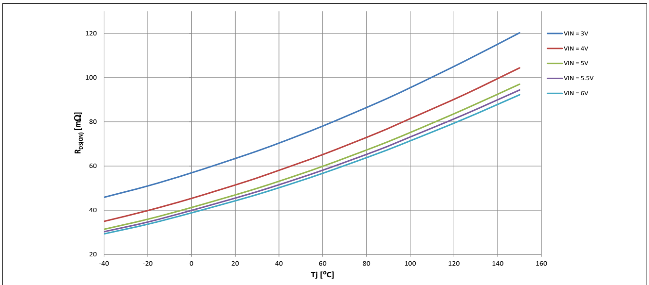
Figure 18 Typical R_{DS(on)} vs. T_J @ V_{IN} = 3V, 4V, 5V, 5.5V, 6V , I_L = 3A
