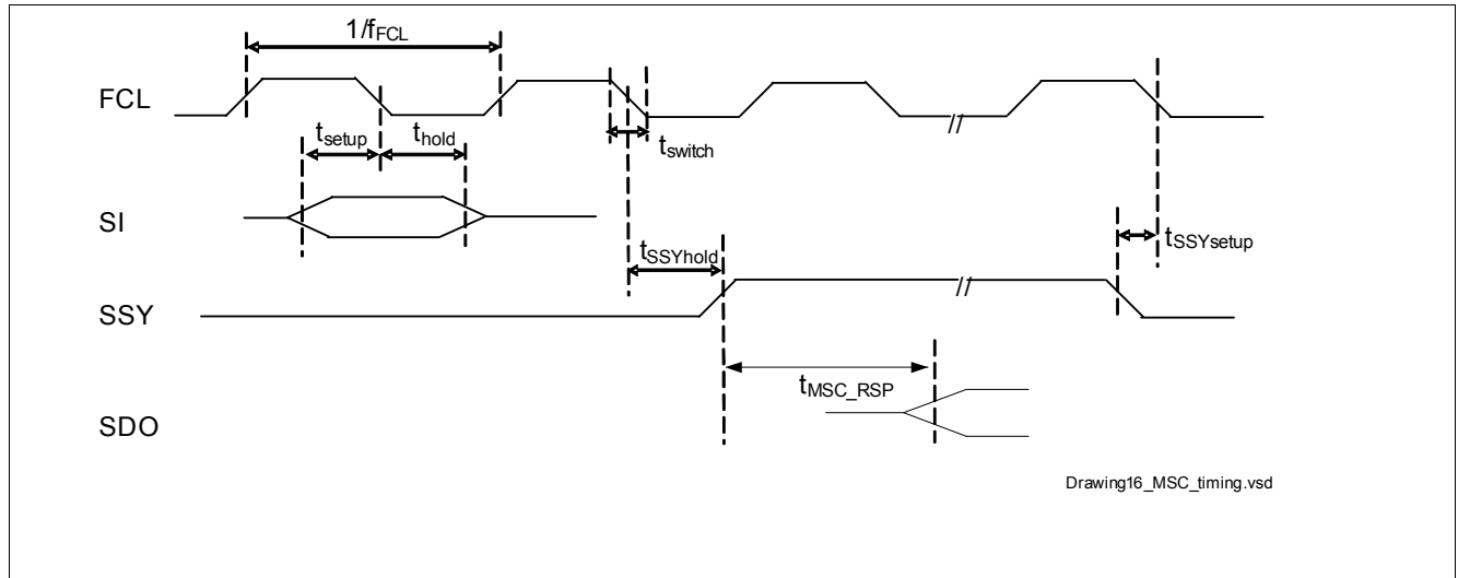
Figure 23 MSC timing
