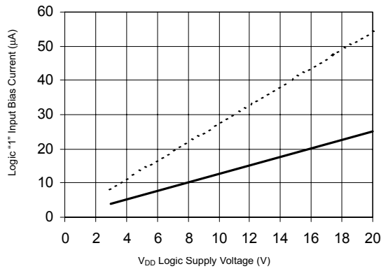
Figure 20B. Logic "1" Input Current vs. V_{DD} Voltage
