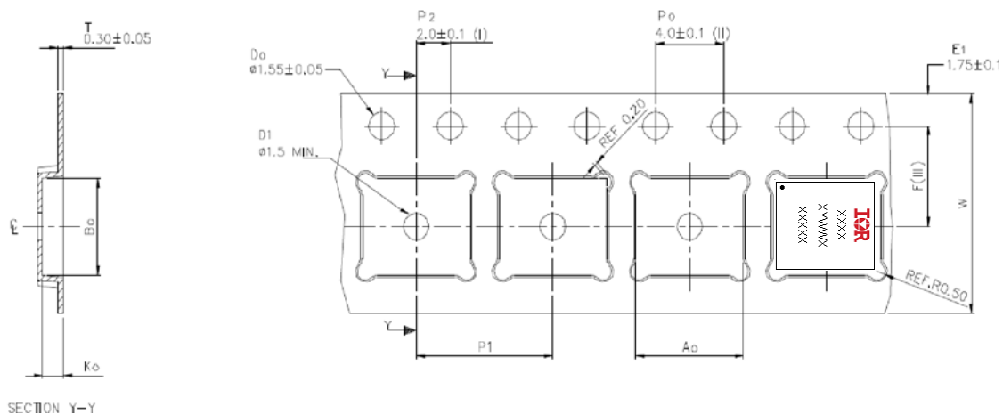
SECTION Y-Y
