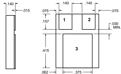
OM1324NMM Pin 1 - Adjust Pin 2 - Input Pin 3 - Output
