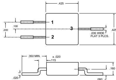
OM1324SMM Front View Pin 1 - Adjust Pin 2 - Input Pin 3 - Output Case - Isolated
