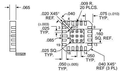
OM1324N2M Pin 1 V OUT (Sense) Pin 11 NC Pin 2 NC Pin 12 NC Pin 3 NC Pin 13 NC Pin 4 NC Pin 14 NC Pin 5 V IN Pin 15 NC Pin 6 NC Pin 16 NC Pin 7 NC Pin 17 NC Pin 8 NC Pin 18 NC Pin 9 NC Pin 19 NC Pin 10 ADJUST Pin 20 V OUT
