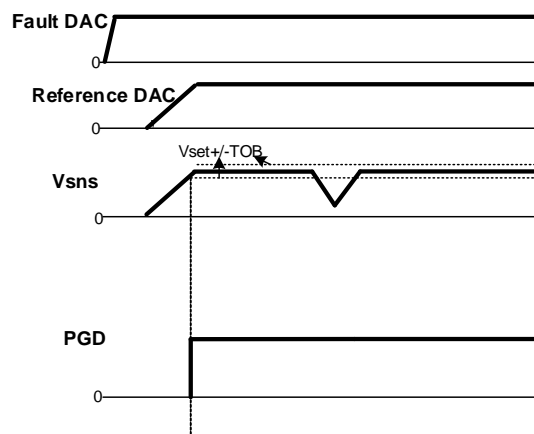
Figure 20: Power Good in PVID mode, Vboot > 0 V
