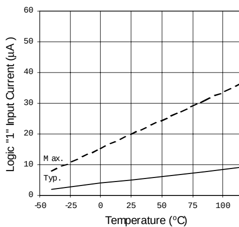
Figure 21A. Logic "1" Input Current vs. Temperature
