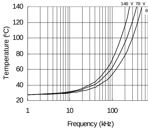
Figure 45. IRS21094S vs. Frequency (IRFBC40), R_{gate}=10\ \Omega , V_{cc}=15\ V
