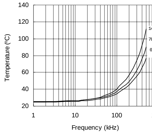
Figure 39. IRS2109S vs. Frequency (IRFBC30), R_{gate}=22\ \Omega , V_{CC}=15\ V
