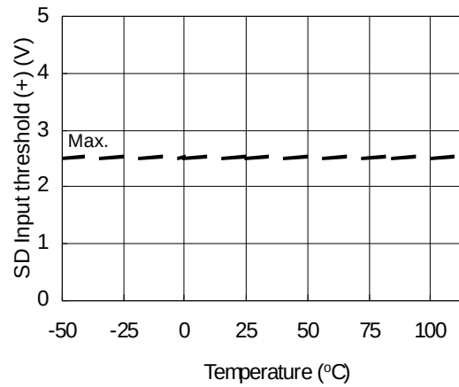
Figure 14A. SD Input Positive Going Threshold (+) vs. Temperature
