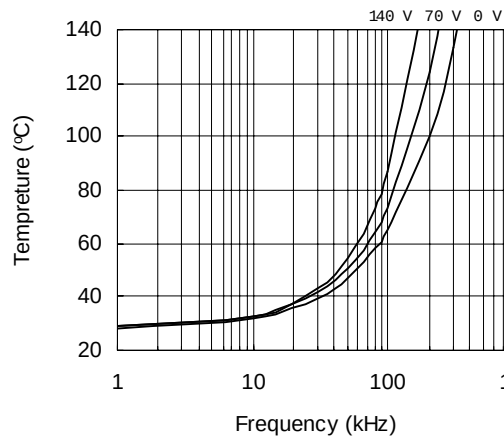
Figure 41. IRS2109S vs. Frequency (IRFPE50), R_{gate}=10\ \Omega , V_{CC}=15\ V
