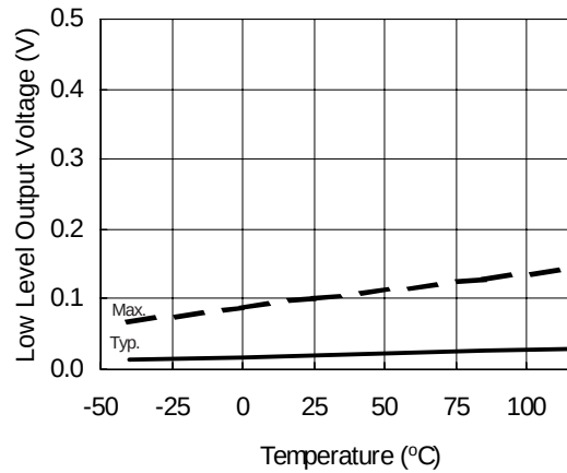
Figure 17A. Low Level Output Voltage vs. Temperature
