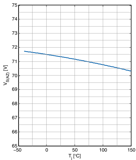
Clamping Voltage V_{S(AZ)} versus Voltage T_j
