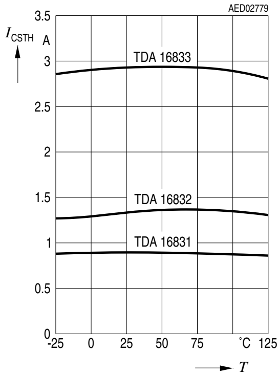
I_{source} Current Limit Threshold I_{csth} versus Temperature
