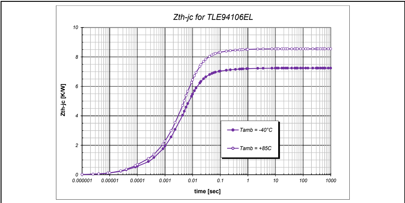
Figure 30 ZthJC Curve
