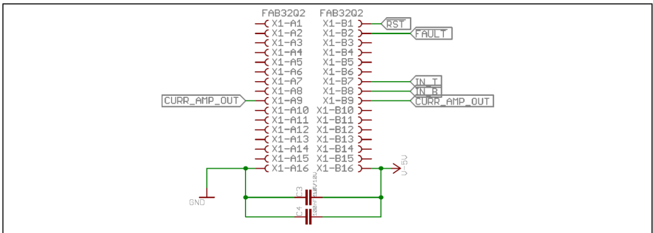
Figure 15 Connector X1
