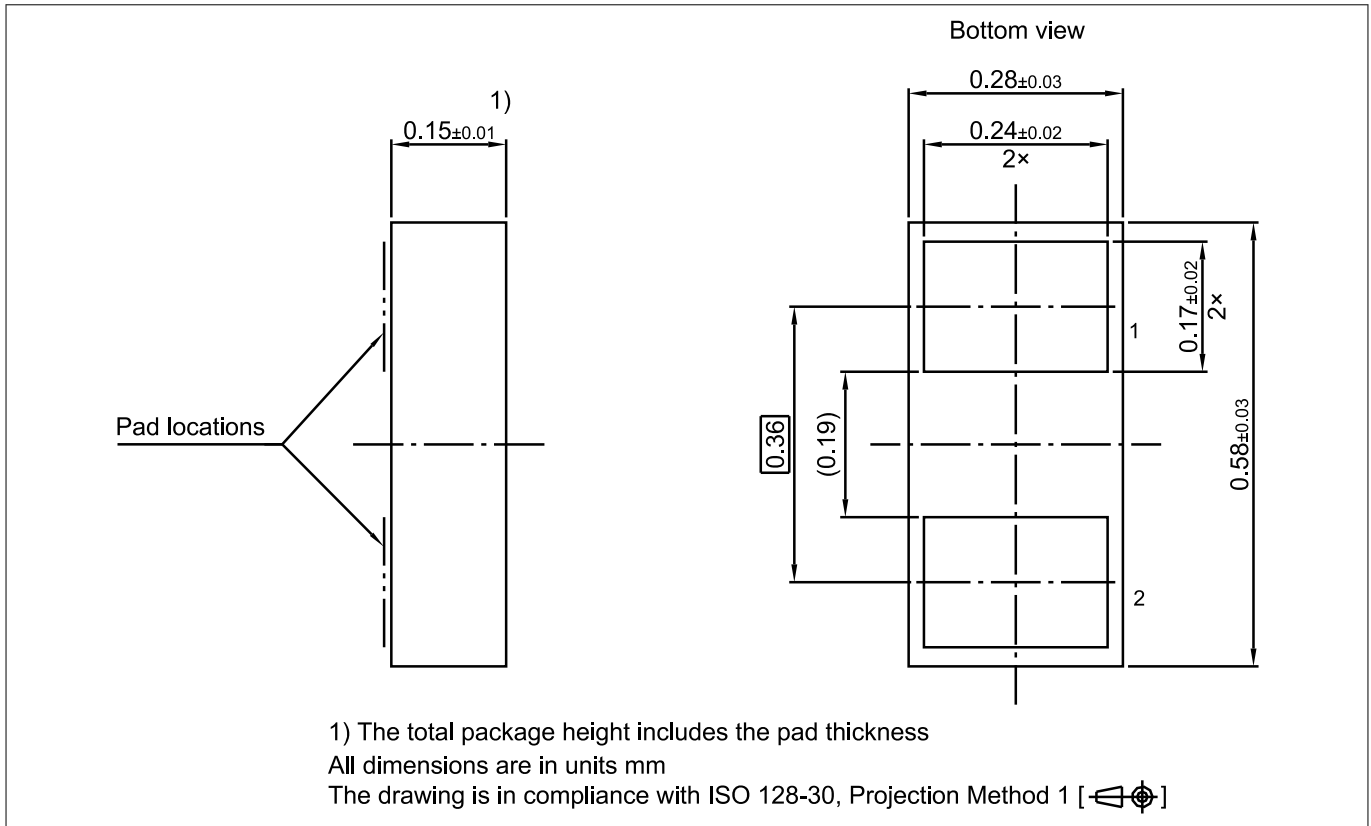
Figure 14 WLL-2-3 package
