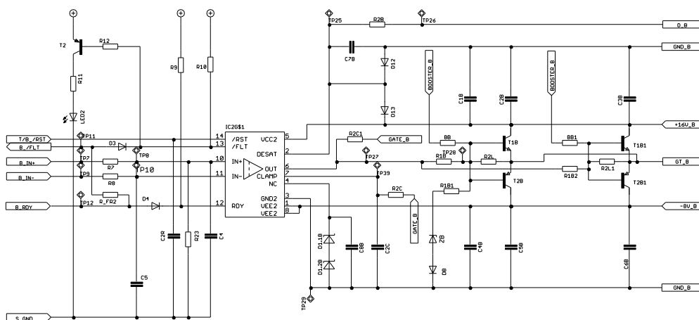
Figure 29 Low side IGBT driver
