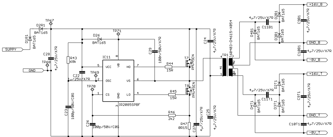
Figure 23 DC/DC converter
