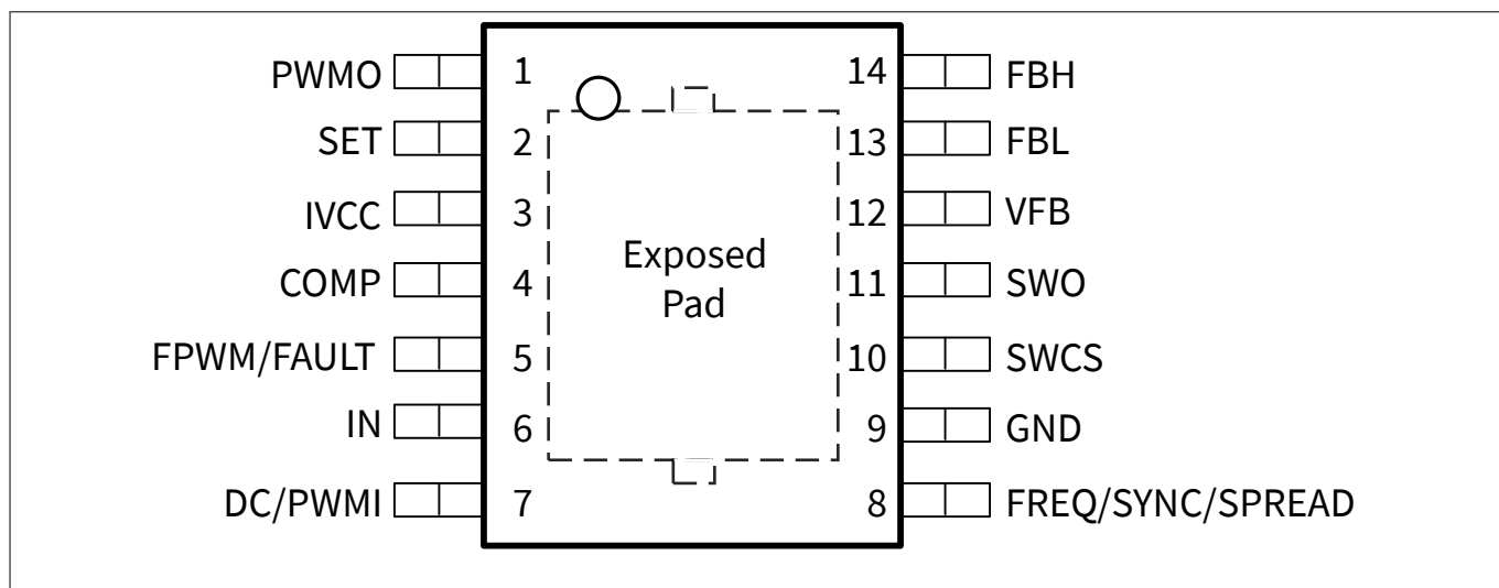
Figure 3 Pin configuration PG-TSDSO-14
