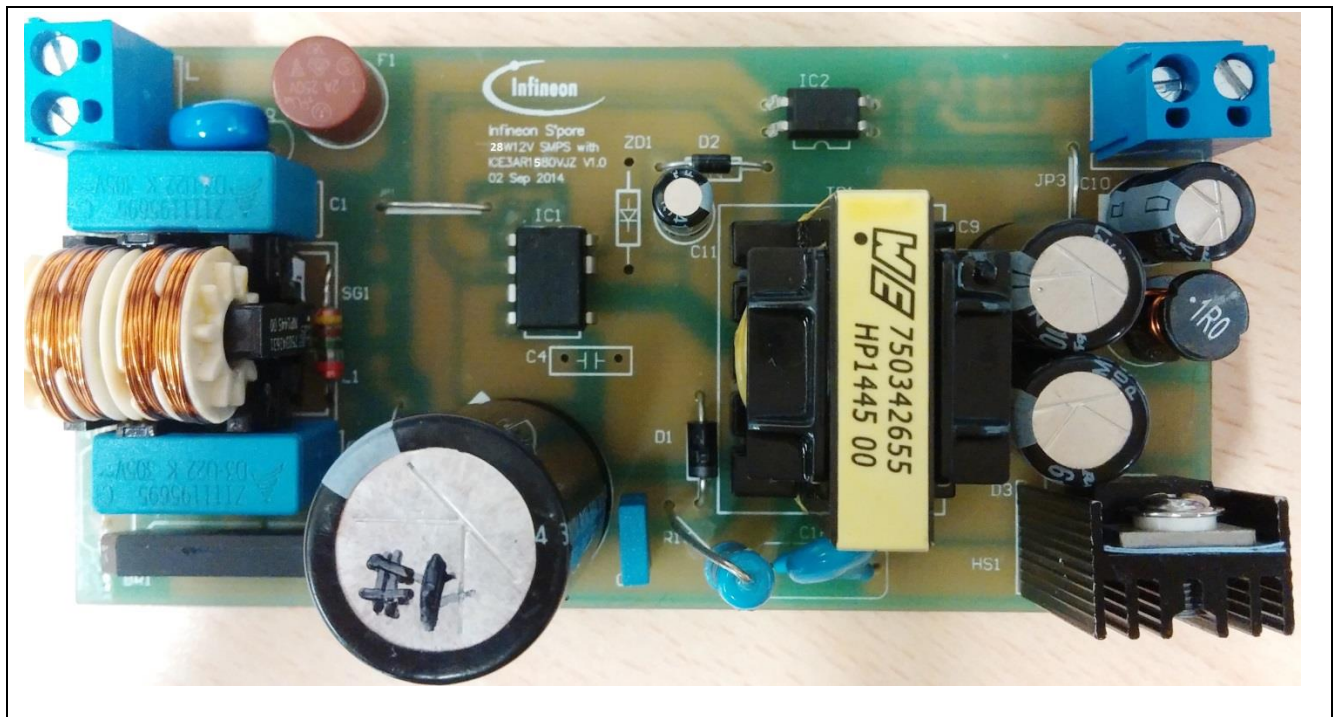
Figure 1 EVAL ICE3AR1580VJZ
