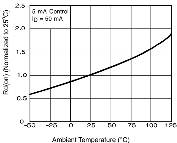
Figure 2. Typical On-Resistance
