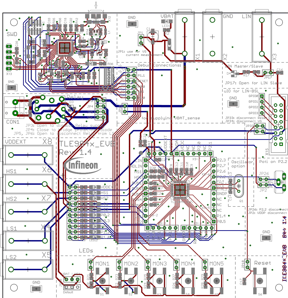
Figure 9 Full Layout
