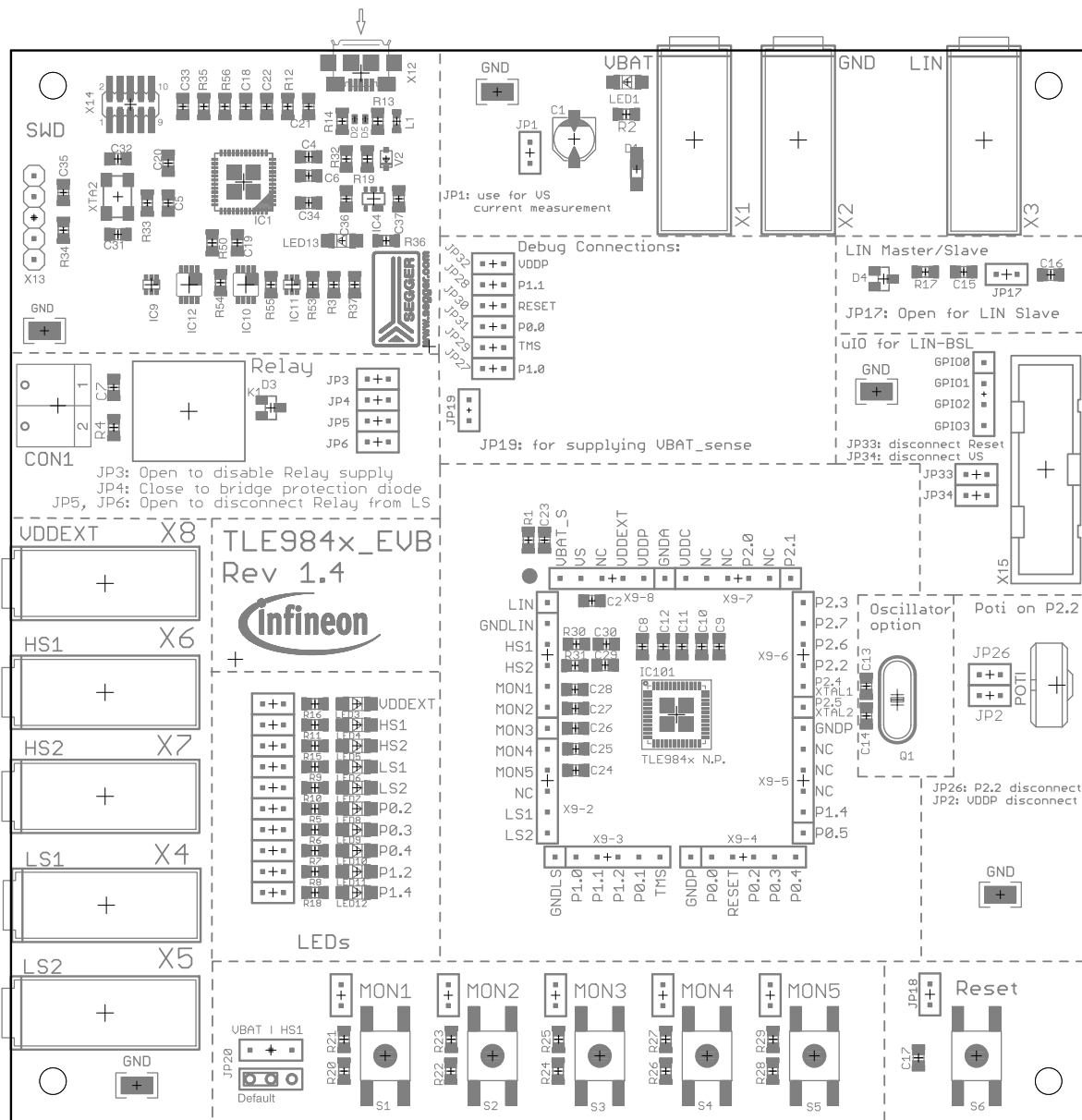
Figure 8 Parts placement
