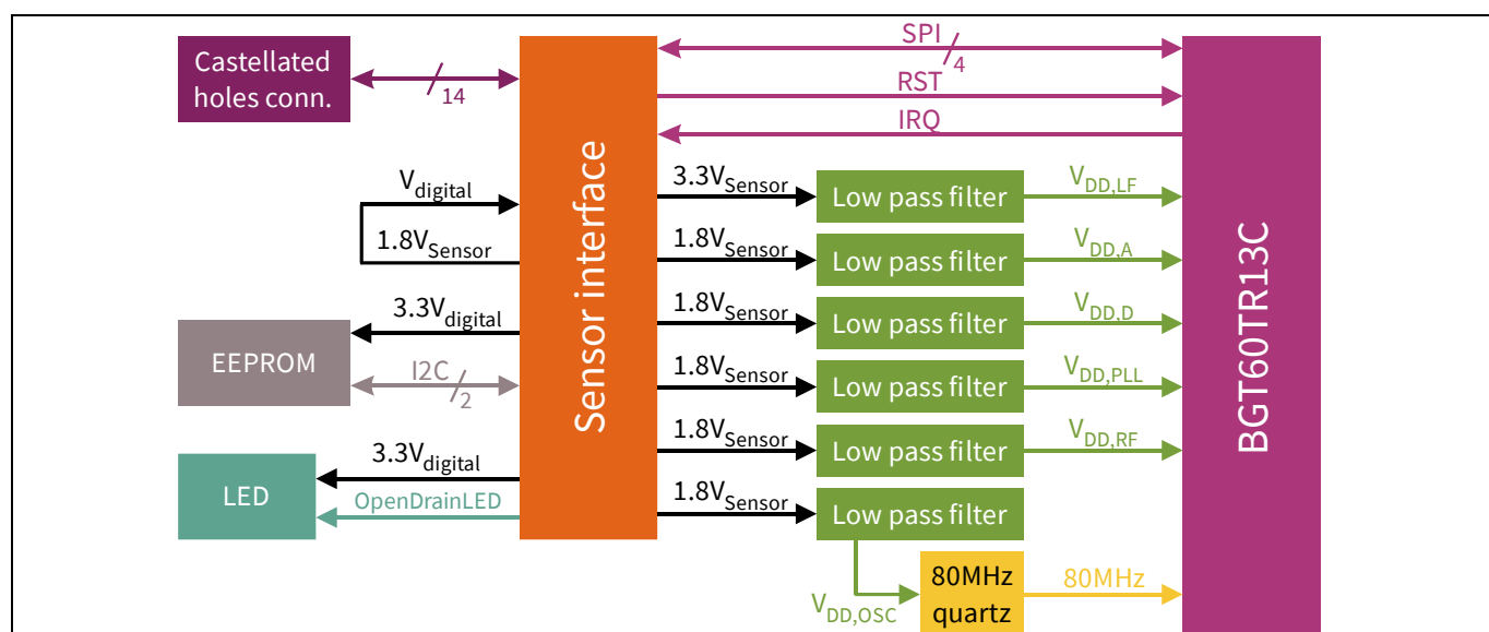
Figure 3 Block diagram of the BGT60TR13C shield
