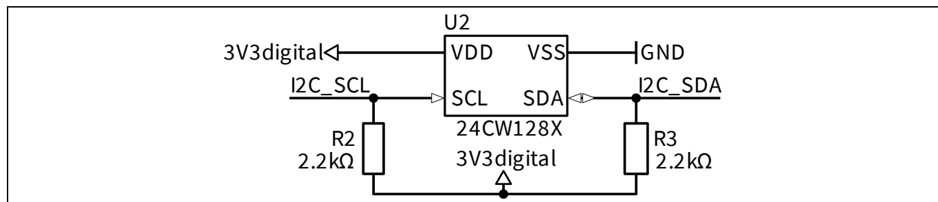
Figure 11 Schematics of the EEPROM
