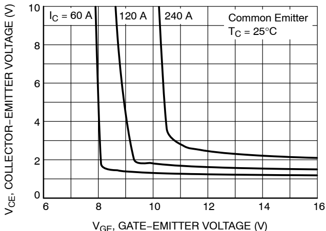
Figure 7. Saturation Voltage vs. V_{CE}
