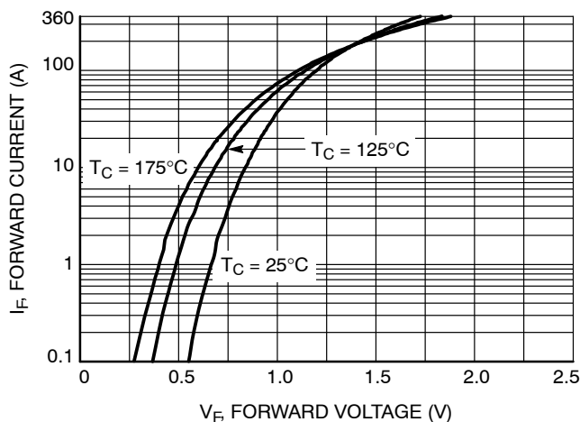
Figure 18. Forward Characteristics
