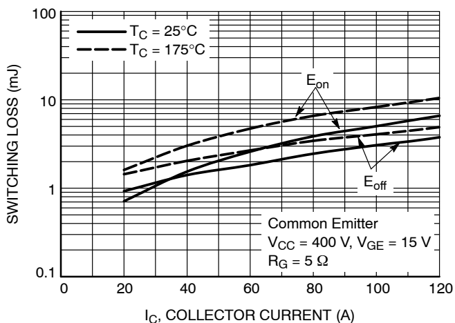
Figure 17. Switching Loss vs. Collector Current
