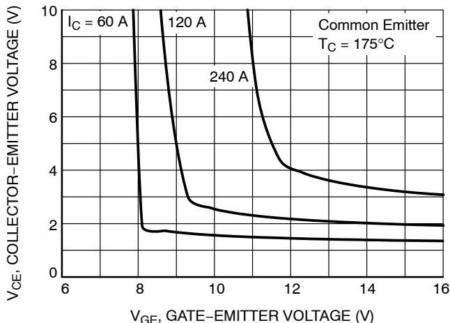
Figure 8. Saturation Voltage vs. V_{CE}
