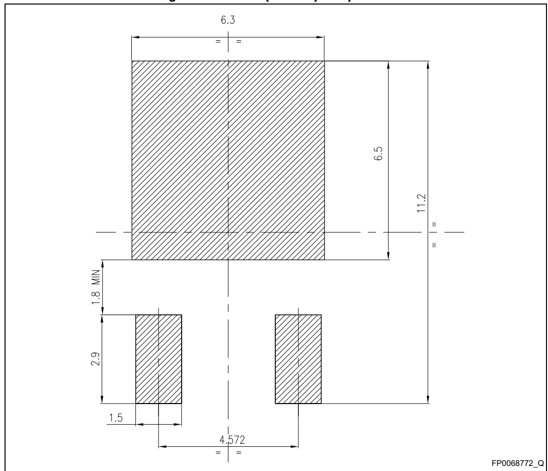
Figure 24. DPAK (TO-252) footprint (b)
