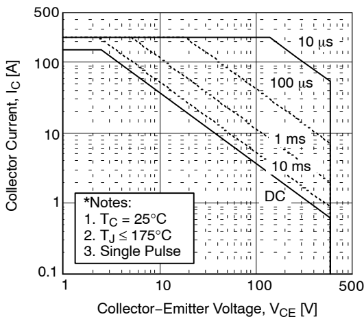
Figure 11. SOA Characteristics
