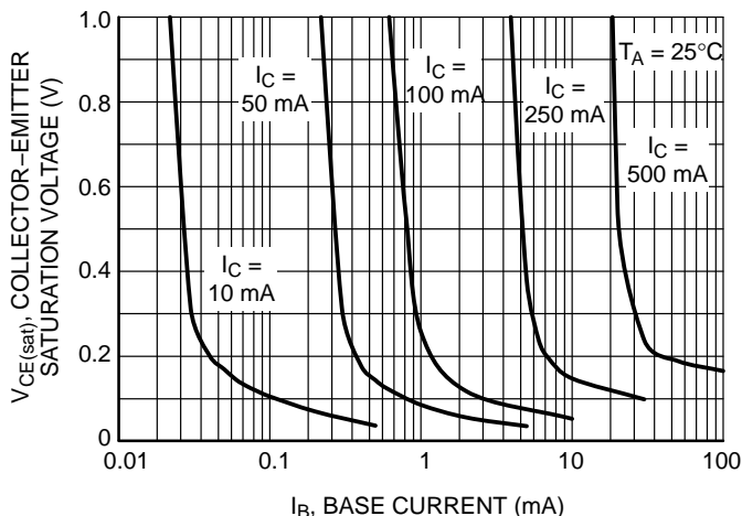
Figure 9. Saturation Region
