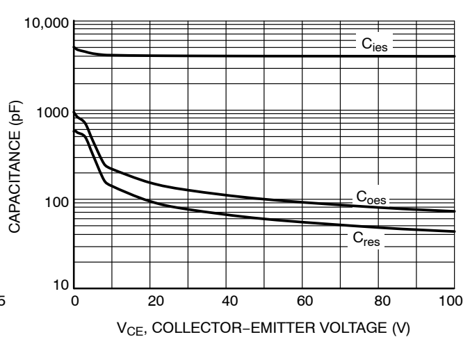
Figure 6. Typical Capacitance
