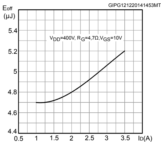
Figure 11. Turn-off switching energy vs drain current
