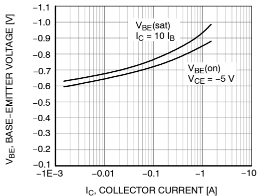
Figure 3. Base-Emitter Voltage
