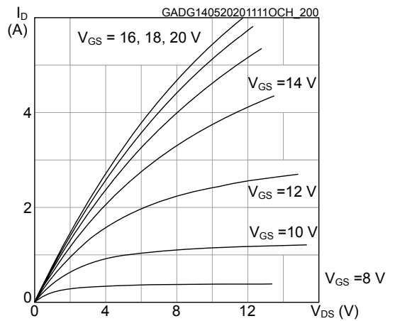
Figure 4. Typical output characteristics (T J = 200 °C)
