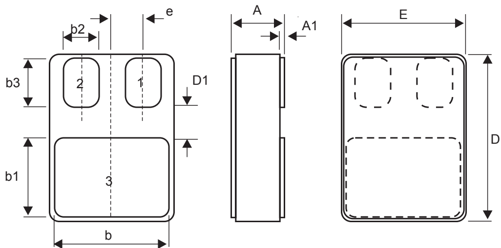
Figure 6. Surface mount SMD.5 package outline (3-terminal)
