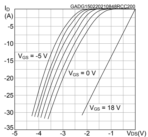
Figure 16. Typical reverse conduction characteristics ( T_J = 200^\circ\text{C} )
