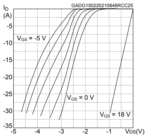
Figure 15. Typical reverse conduction characteristics ( T_J = 25^\circ\text{C} )
