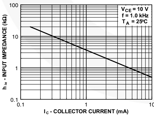
Figure 17. Input Impedance
